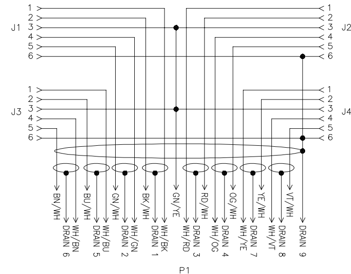
WIRING DIAGRAM
